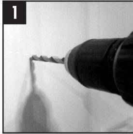
1 Drill hole in fiberglass using 5/16"
